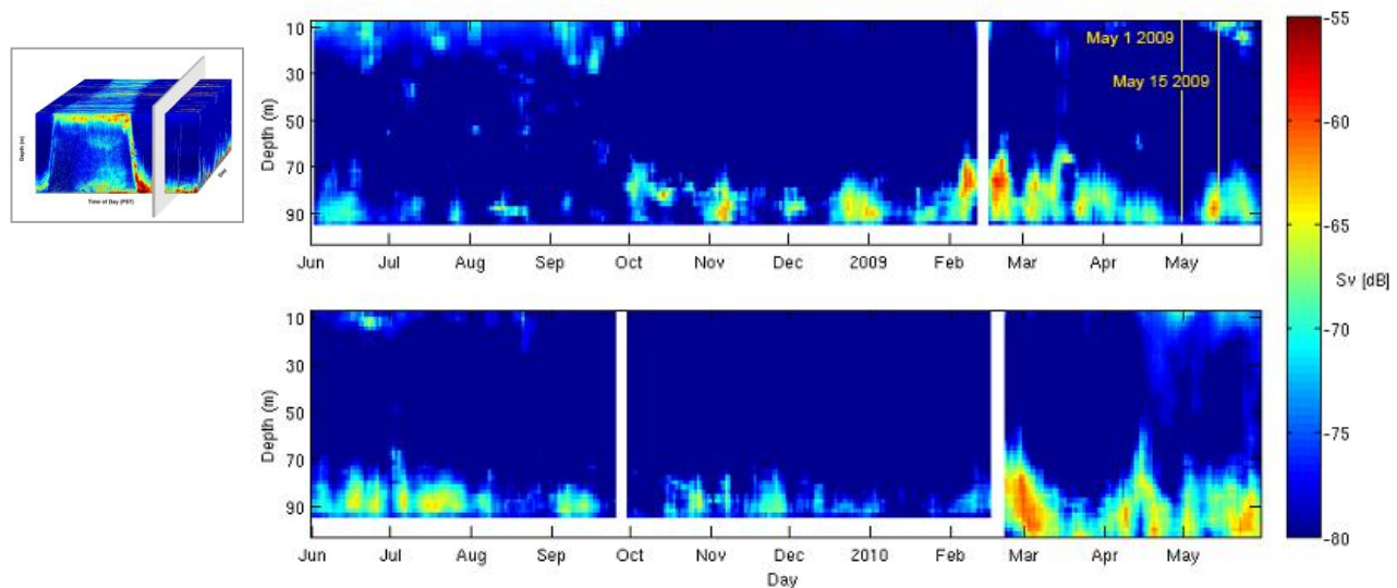
Fig. 3. Echograms of S_v (dB) at noon (12:00 PST) for the period June 1, 2008 – May 31, 2010. A change in recording depth at the end of February 2010 was due to the redeployment of the AWCP at a nearby location but 10 m deeper. The inset illustrates the orientation of the data slice depicted relative to the data cube. High temporal resolution echograms for May 1 and 15, 2009 are shown in Fig 4.
