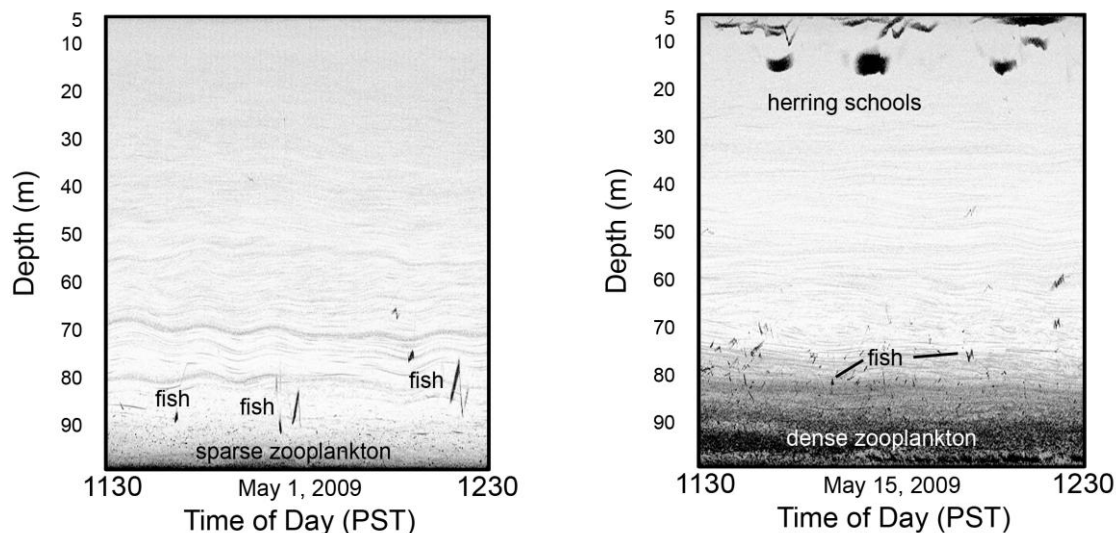
Fig. 4. High temporal resolution plots around noon on May 1 and 15, 2009, illustrating the differences captured in the plot in Fig. 3.
